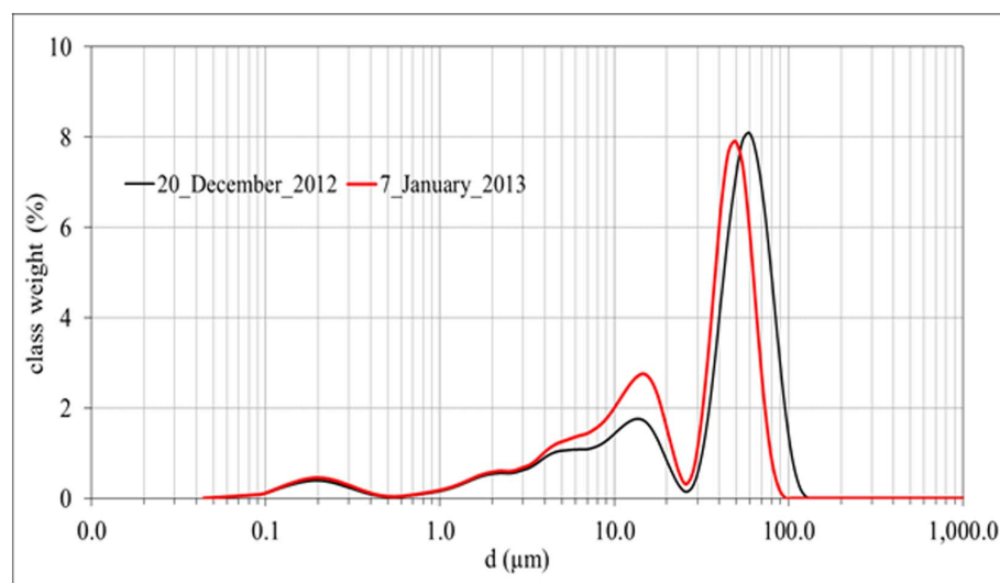
Figure 2 | Particle size distribution of the dust samples by a high-resolution laser diffractometer technique (ANALYSETTE 22 MicroTec Plus), with the statistical parameters.
