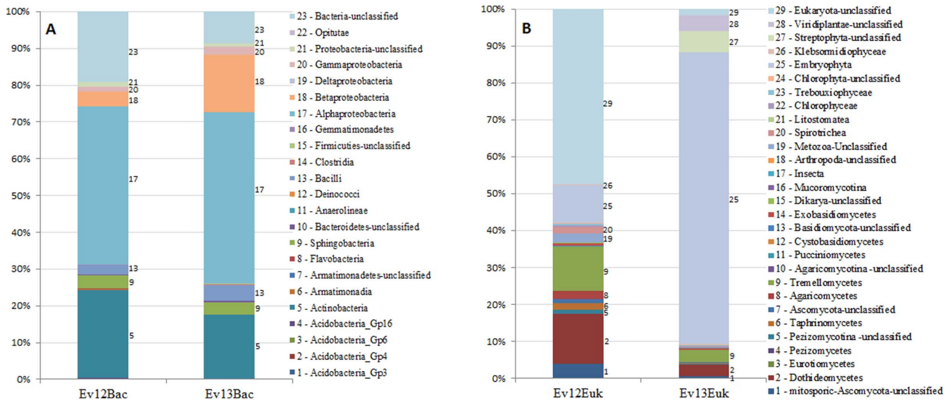
Figure 3 | Distributions of rRNA genes reads, retrieved from the dust samples Ev12 and Ev13. (a) Bacterial 16S reads at the class level. Affiliation of classes to different phyla are: 1–4 Acidobacteria ; 5 – Actinobacteria ; 6–7 – Armatimonadetes ; 8–10 – Bacteroidetes ; 11 – Chloroflexi ; 12 – Deinococcus-Thermus ; 13–15 – Firmicutes ; 16 – Gemmatimonadetes ; 17–21 – Proteobacteria ; 22 – Verrucomicrobia ; 23 – unclassified. (b) Eukaryotic 18S reads at the kingdom-class levels. Affiliation of taxonomic categories to highest taxonomic ranks are: 1–16 – Fungi kingdom (1–7 – Ascomycota phylum; 8–14 – Basidiomycota phylum; 15 – unclassified Dikarya superphylum; 16 – Basal fungal lineages phylum); 17–19 – Metazoa kingdom (17–18 – Arthropoda phylum; 19 – unclassified Metazoa ); 20–21 – Alveolata superphylum ( Ciliophora phylum); 22–28 – Viridiplantae phylum; 29 – unclassified eukaryota phylum.
