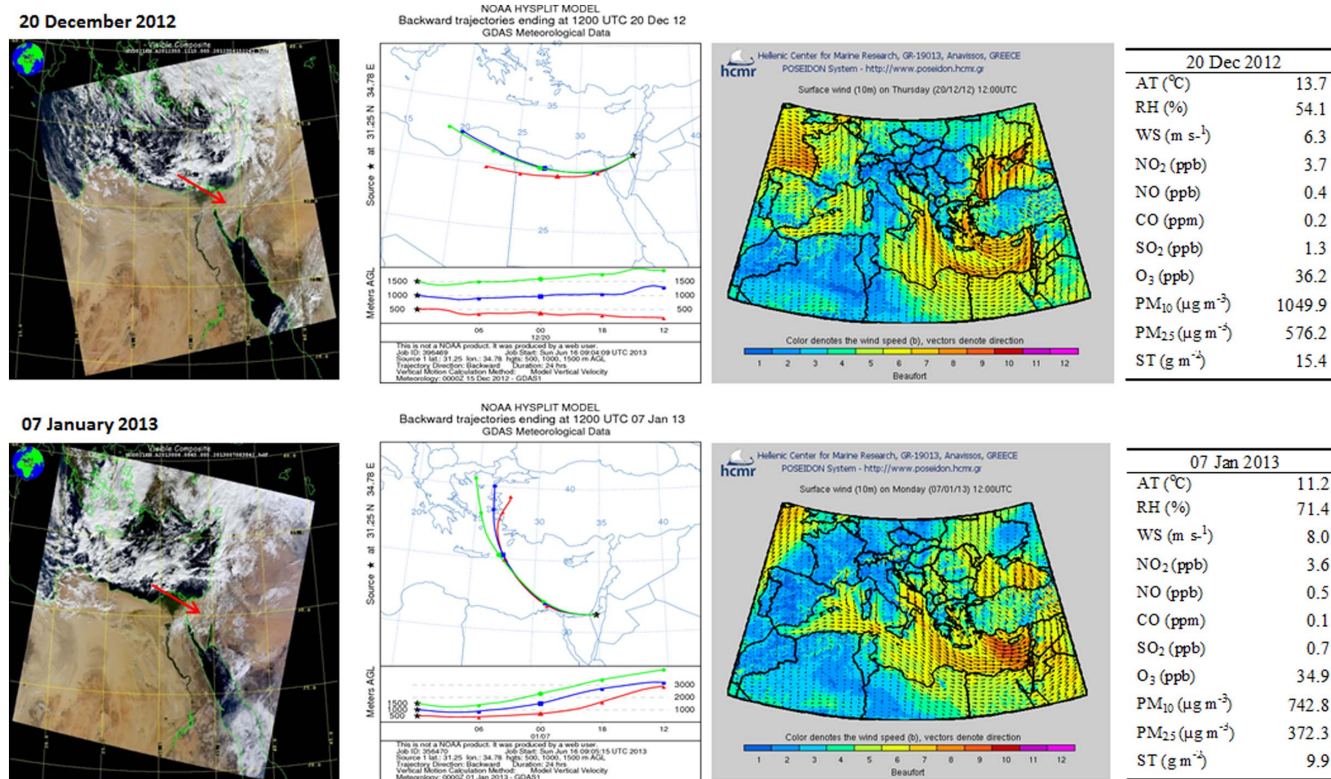
Figure 1 | Satellite images (MODIS) of the studied region during the dust storms along with air mass transport at different heights above ground level (AGL) derived from Backward Trajectories model NOAA/ARL HYSPLIT-4 (credit to: www.noaa.gov ) and equivalent wind directions at 10 m above surface level from the HCMR POSEIDON System (credit to: www.poseidon.hcmr.gr ). Red arrowheads indicate the sampling site. Right hand side panels: daily recorded averages of major meteorological variables and pollutants. AT – air temperature; RH – relative humidity; WS – wind speed; PM – particulate matter; ST – settled dust.
