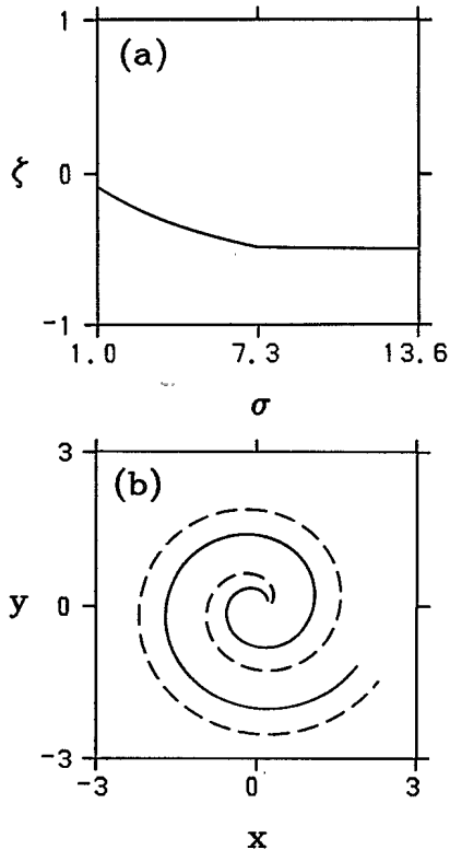
FIG. 3. (a) Asymptotic profile of \zeta obtained by numerical integration of (8). Parameter values used are \rho_0=0.2 , \sigma_{\min}=1.0 , \omega=0.7 , D=0.002 , a_R=-a_L=1.0 , \eta_R=10.0 , \eta_L=3.0 , and v_L=\phi_L=0.0 . (b) Asymptotic spiral (solid curve) and involute spiral (dashed curve) for the parameters of (a).
