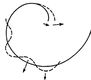
FIG. 1. Schematic illustration of the effect of curvature. Normal velocity (indicated by arrows) decreases as curvature increases. As a result small perturbations (dashed curves) that occur significantly far from the tip always decay, while those involving the tip may grow.
