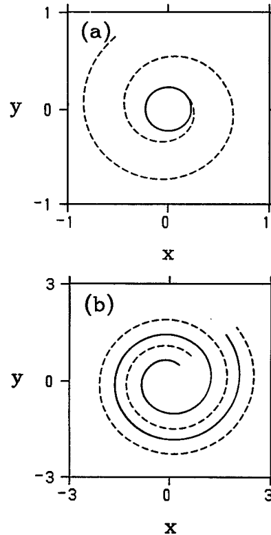
FIG. 4. (a) Dynamics of spiral tips. Steady circular motion obtained with a monotonic tail (solid curve) vs an outward spiral motion obtained with an oscillatory tail (dashed curve). Parameter values are as in Fig. 3 except that v_L=2.0 in the latter case. (b) Demonstration of core expansion. Spiral wave at an early stage (solid curve) and at a later time with larger core (dashed curve). Parameter values are as in Fig. 3 except that v_L=2.0 .
