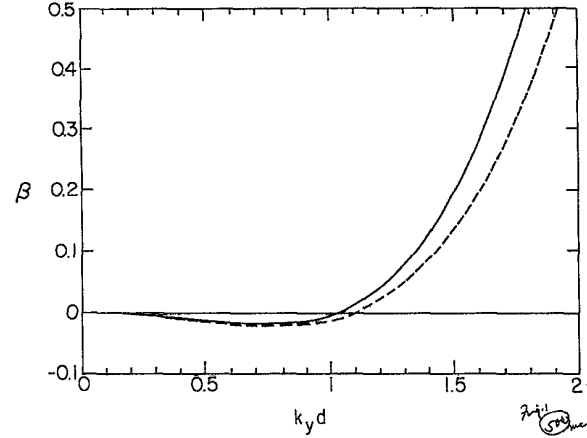
FIG. 1. A graph of the coefficient \beta in Eq. (6) as a function of k_y d where the depth d of the cell has been taken to be 2 cm. The solid and the dashed curves correspond, respectively, to zero surface tension and to surface tension of water.
