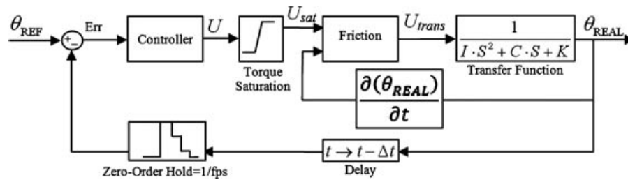
Figure 8. A simplified (one-DOF) system model used in our analysis.
