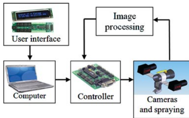
Figure 5. The control architecture of the spraying system.
