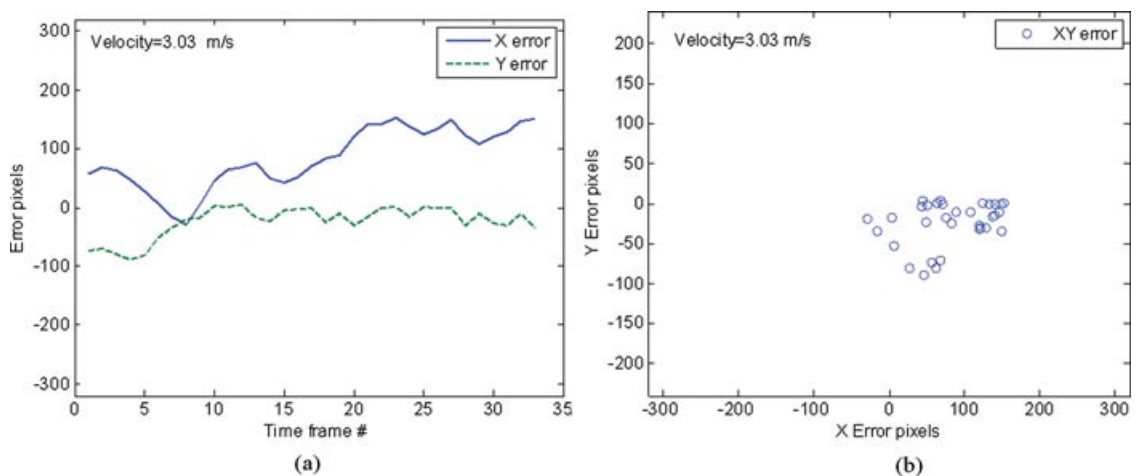
Figure 18. Typical behavior of the tracking error in both the x and y directions for speeds that are higher than 1.25 m/s. (a) Changes in the tracking error as a function of time. (b) The tracking error in compression to the image frame.
