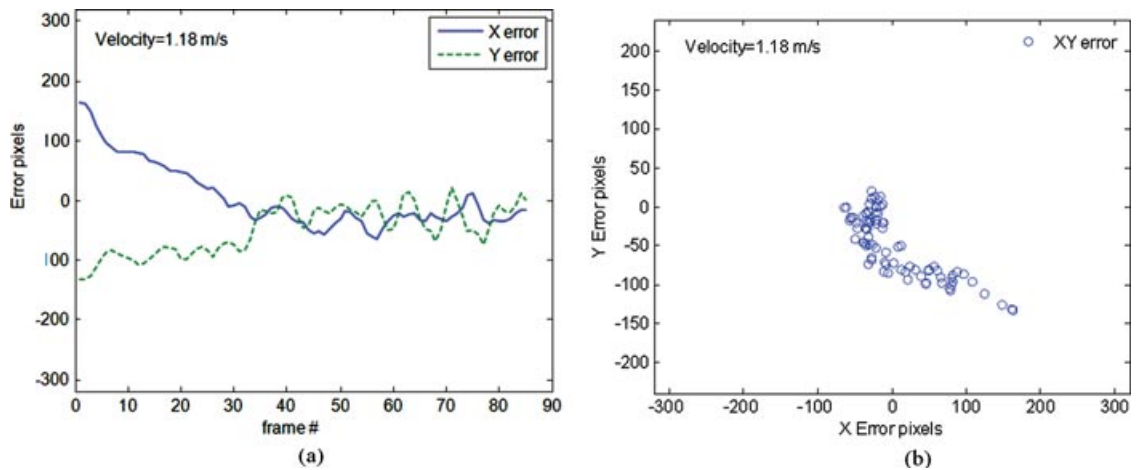
Figure 17. Typical behavior of the tracking error in both the x and y directions for spraying velocities that are lower than 1.25 m/s. (a) Tracking error as a function of time. (b) Distribution of target positions in the image plane (note that the larger errors are a result of the initial offset with which the trial was initiated).
