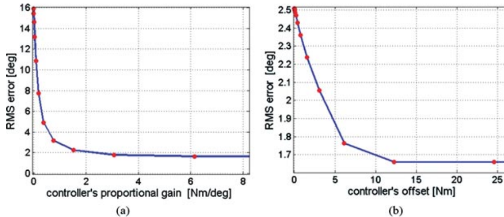
Figure 10. RMS angular error of the spraying head (a) as a function of the controller's proportional gain ( K_p ) and (b) as a function of the controller's offset parameter C_p . Both graphs were computed for a wagon velocity of 1.2 m/s.
