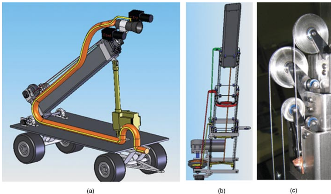
Figure 3. (a) The folded sprayer mounted on a wagon. (b) The open telescopic mast and the winch. (c) Pulley and cable system of the folded telescopic mast.
