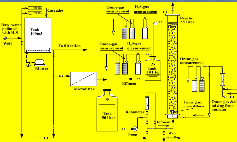
Ozonization treatment system for the removal of hydrogen sulfide from water of wells
