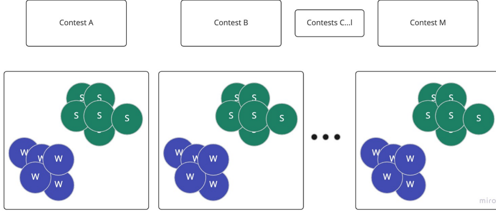
Figure 2: m contests, each comprising of strong (S) and weak (W) agents.
