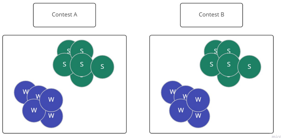
Figure 1: Two contests, each comprising of strong (S) and weak (W) agents.
