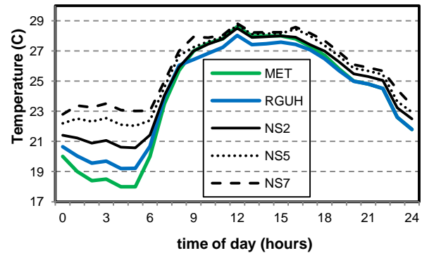
Figure 1: Dry bulb temperature at the weather station (MET), simulated hydrological effects on air temperature (rural geometry urban hydrology, RGUH) and predicted temperatures for a N-S street canyon flanked by buildings of 2, 5 and 7 storeys.
