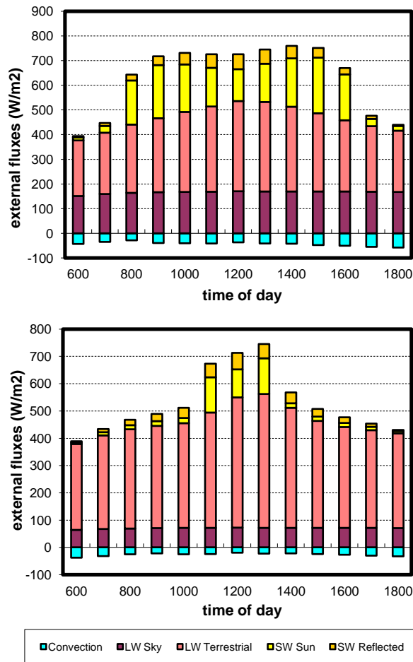
Figure 3: Breakdown of fluxes causing thermal stress on a pedestrian in a N-S canyon with 2-storey buildings (top) and 7 storeys (bottom).
