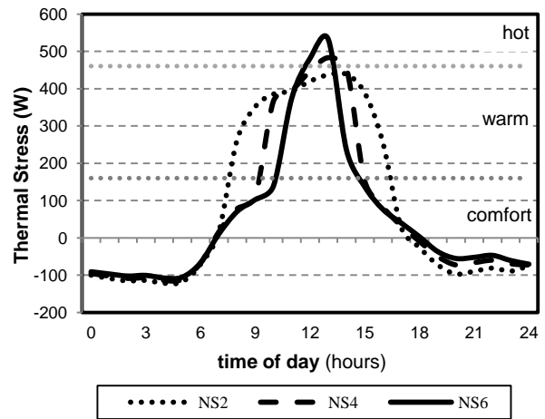
Figure 4: Pedestrian thermal stress (W) for a N-S street canyon of 2, 4 and 6 storeys. ITS categories: <160W “comfortable” (ITS=4); 160-460W “warm”(ITS=5); 460-760W “hot” (ITS=6); >760 “very hot”(ITS=7).
