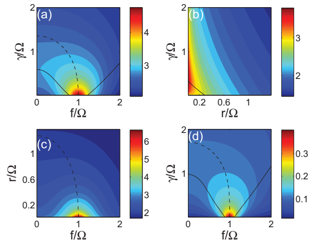
Fig. 1: (Colour on-line) (a) Mean surface current speed (in cm/s) as a function of the Coriolis parameter (frequency), f , and the temporal correlation parameter, \gamma . (b) Same as (a) but for the friction parameter r and temporal correlation parameter \gamma . (c) Same as (a) but for the friction parameter r and the Coriolis parameter f . (d) Same as (a) but for the current at a depth of 400 m. In all panels, the solid line indicates the maximum value along the vertical axis while the dashed line indicates the maximum value along the horizontal axis. Parameter values are: \Omega = 2\pi/86400 \text{ s}^{-1} , f = 2\Omega \sin(45^\circ) , \omega_0 = \Omega , \tau_0 = 0.1 \text{ N m}^{-2} , \nu = 0.1 \text{ m}^2 \text{ s}^{-1} , \rho_0 = 1028 \text{ kg m}^{-3} , r = 10^{-5} \text{ s}^{-1} , \gamma = 10^{-5} \text{ s}^{-1} .
