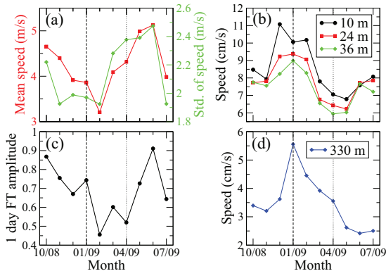
Fig. 2: (Colour on-line) (a) Monthly mean (red) and standard deviation of the wind speed (in m/s) from the Gulf of Elat ( 34.92^{\circ}\text{E} , 29.5^{\circ}\text{N} ). (b) Monthly mean current speed (in cm/s) at different shallow depths. (c) FT amplitude of the wind speed at the diurnal frequency. (d) Monthly mean current speed (in cm/s) at a depth of 330 m. The vertical dashed line indicates January 2009 and the vertical dotted line indicates April 2009.
