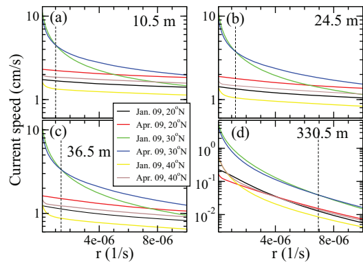
Fig. 3: (Colour on-line) Mean simulated current speed as a function of the friction coefficient, r , when forced by the observed winds of January and April 2009 from the Gulf of Elat, for different latitudes ( 20^{\circ}\text{N} , 30^{\circ}\text{N} , and 40^{\circ}\text{N} ) and depths: (a) 10.5 m, (b) 24.5 m, (c) 36.5 m, and (d) 330.5 m. The vertical dashed line indicates the transition point at which the mean current speed of January 2009 becomes smaller than that of April 2009.
