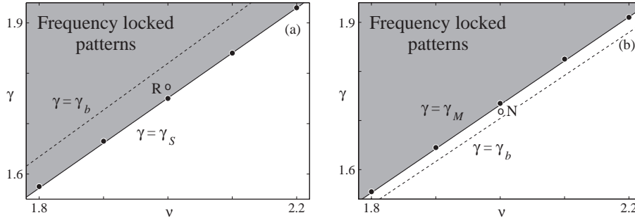
Fig. 5 – The boundaries of resonant patterns as computed from eqs. (10) and (11) (solid lines) vs. the boundaries of resonant uniform oscillations (dashed lines). The solid circles indicate the boundaries obtained from direct numerical solution of eq. (2). Shaded areas denote resonant dynamics. In (a) the effect of the Turing mode is to extend the range of resonant dynamics, whereas in (b) the effect is to reduce it. The points “R” ( \gamma = 1.77 , \nu = 2 ) and “N” ( \gamma = 1.72 , \nu = 2 ) correspond to the resonant and non-resonant patterns shown in figs. 4(a) and (b), respectively. Parameters: \mu = 0.1 , \alpha = 0.5 , and (a) \beta = 0.4 and (b) \beta = 0.55 .
