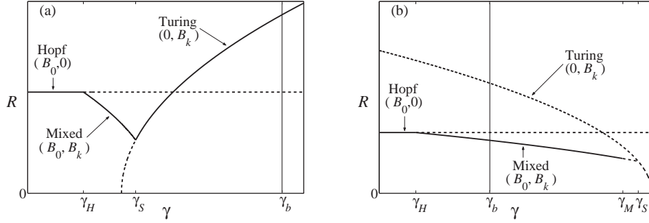
Fig. 3 – Bifurcation diagrams for uniform solutions of eq. (7) showing the existence and stability ranges of the two pure-mode solutions and the mixed-mode solution as the forcing \gamma is varied. The vertical axis is R = \sqrt{|B_0|^2 + |B_k|^2} . The solid (dashed) curves denote stable (unstable) solutions. The thin vertical lines in (a) and (b) highlight the location of the uniform-oscillation boundary, \gamma = \gamma_b . Note that in (b) the uniform-oscillation boundary lies inside the stable mixed-mode region. Parameters: \mu = 0.1 , \nu = 2 , \alpha = 0.5 , (a) \beta = 0.4 and (b) \beta = 0.55 .
