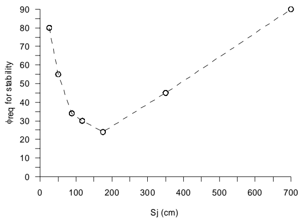
Figure 12: \phi_{\text{req}} for stability vs. joint spacing, and optimal joint spacing for a given layered Voussoir beam 1 .
