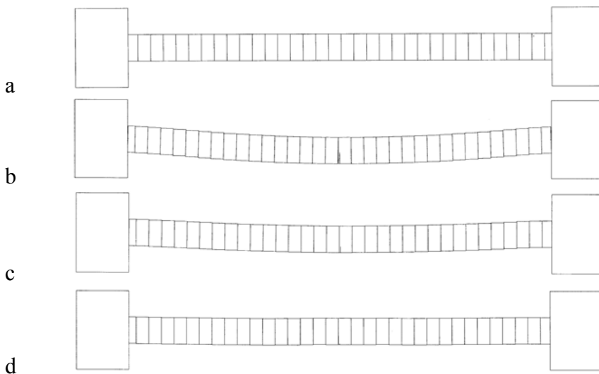
Figure 9. DDA graphic output of single layer deformation for different values of joint friction angle: a) original geometry; b) \phi_{av} = 45^\circ ; c) \phi_{av} = 75^\circ ; d) \phi_{av} = 80^\circ .
