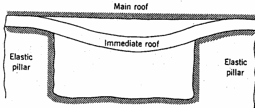
Figure 16. Deflection of a single layer on elastic pillars, after Obert and Duvall 12
