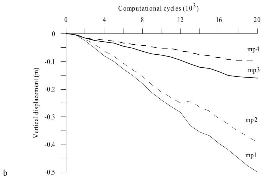
Figure 19. DDA measurement point output (for location see Figure 17b). a) vertical joints configuration, b) inclined joints configuration.
