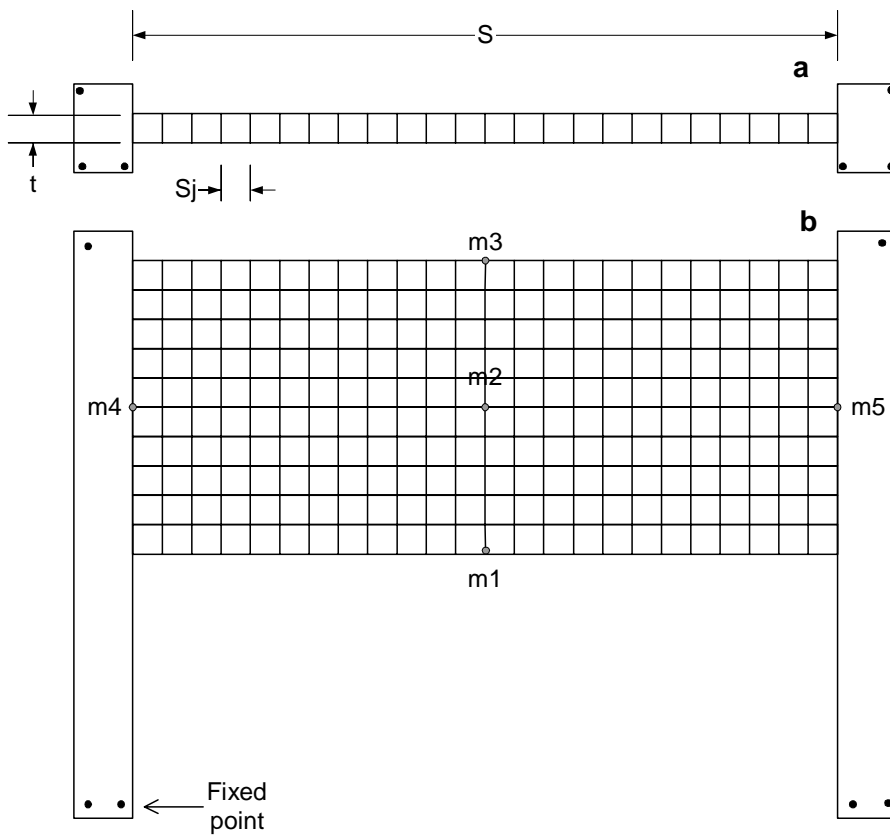
Figure 8. Single layer and multiple layered beam models studied in DDA
